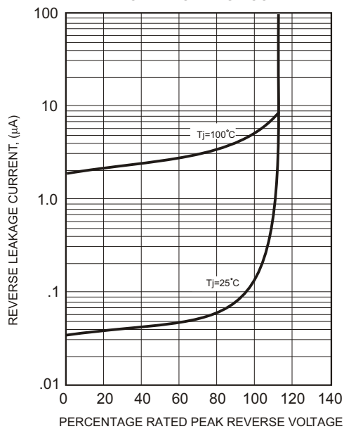
FIG.3 - TYPICAL REVERSE
