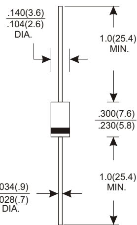
DO-15
