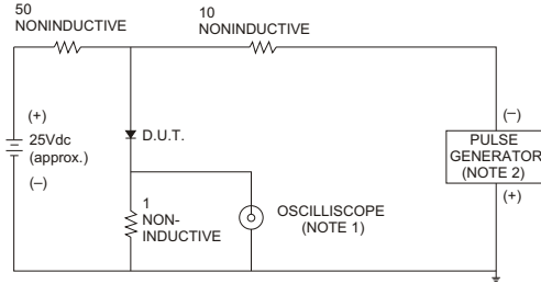
FIG.1- TEST CIRCUIT DIAGRAM AND REVERSE
