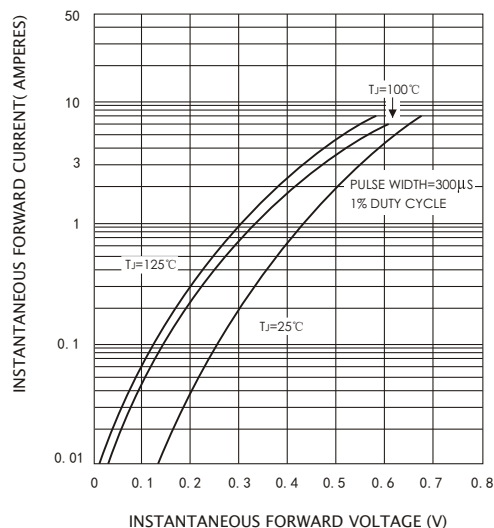
FIG.2-TYPICAL FORWARD CHARACTERISTICS
