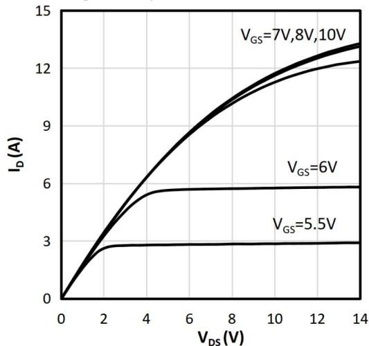
Fig 1: Output Characteristics
