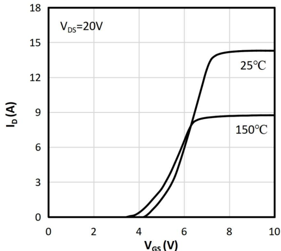
Fig 2: Transfer Characteristics
