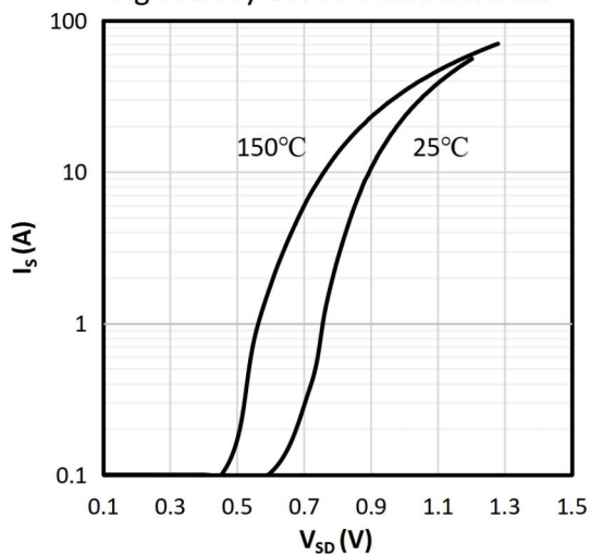
Fig 7: Body-Diode Characteristics
