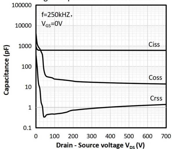
Fig 8: Capacitance Characteristics
