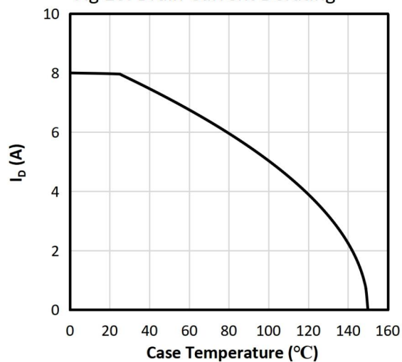
Fig 10: Drain Current Derating
